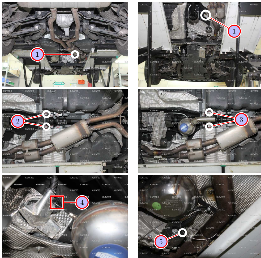
Figure 10: Installation external sound generator Version 3 - Gasoline Engines
