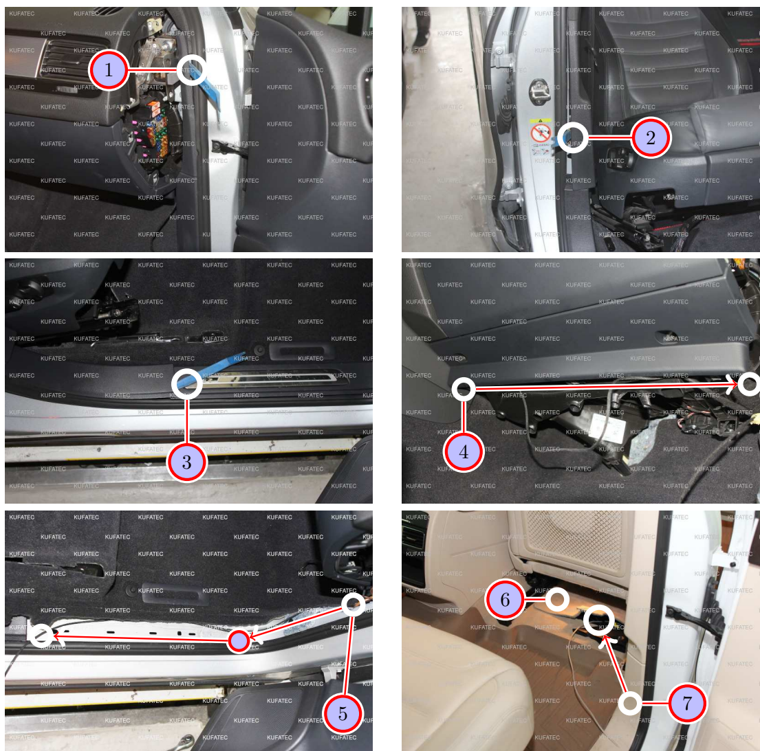
Figure 7: Routing connecting cable external sound generator
