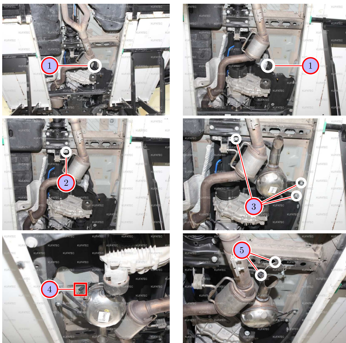
Figure 9: Installation external sound generator Version 2 - 3.0 TDI
