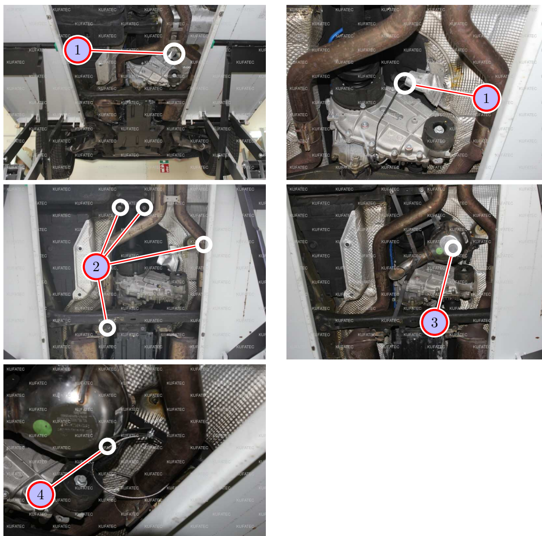
Figure 8: Installation external sound generator Version 1 - 4.3 TDI
