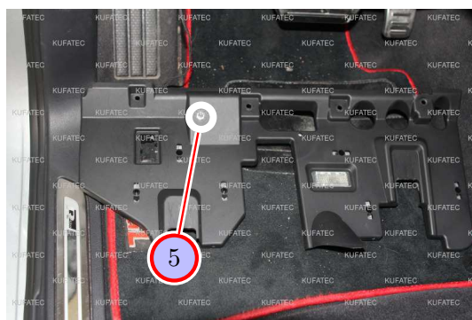
Figure 11: Installation pushbutton
