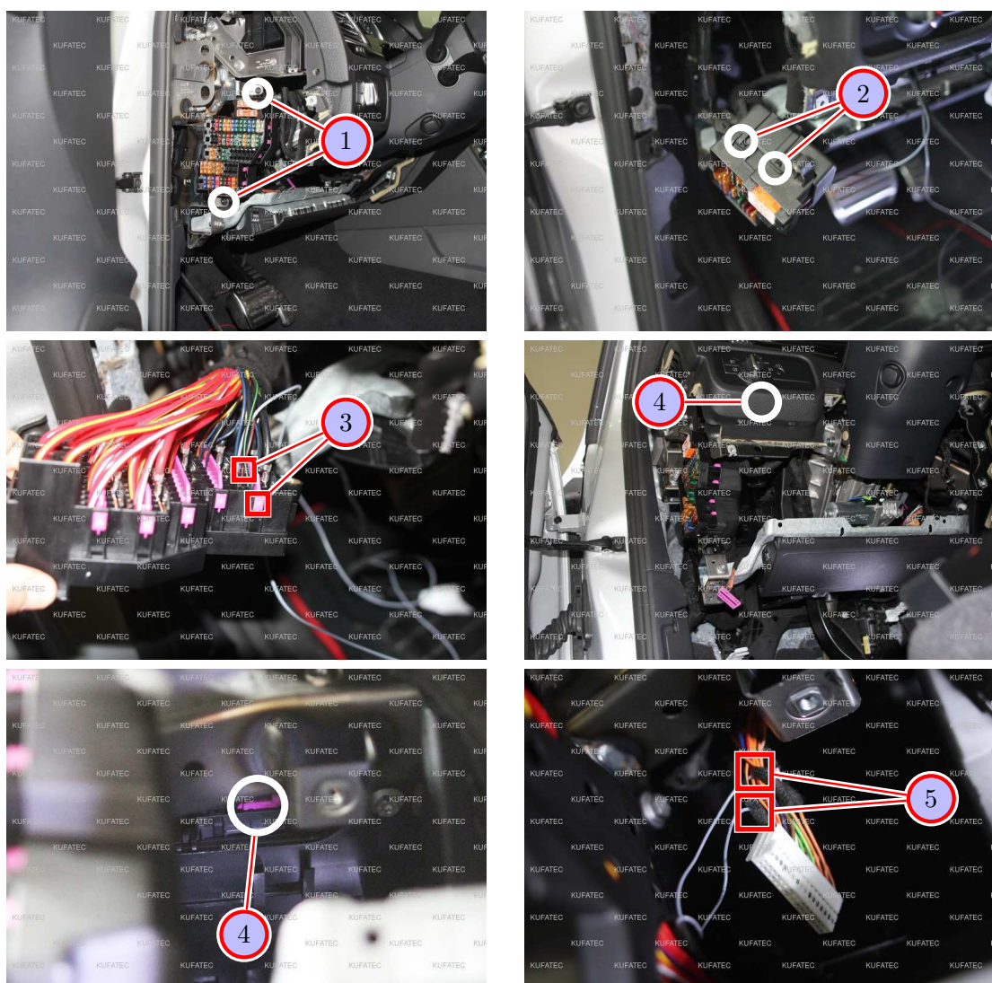
Figure 5: Connection Ignition plus / CAN High & CAN Low
