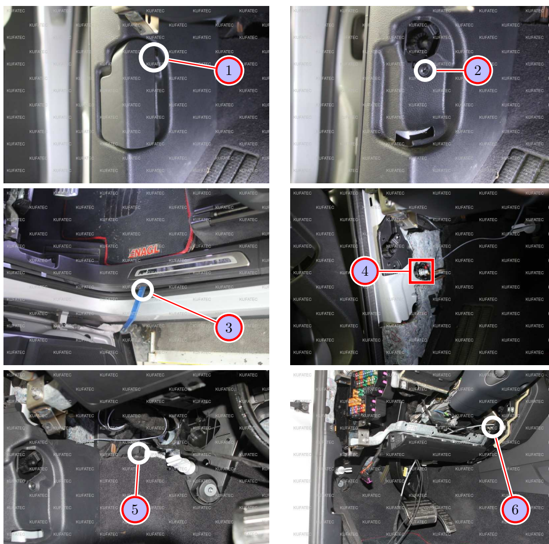
Figure 6: Connection Ground / Laying of cable
