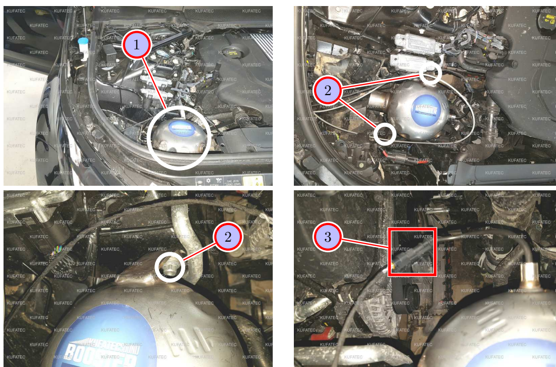
Figure 12: Installation front sound generator
