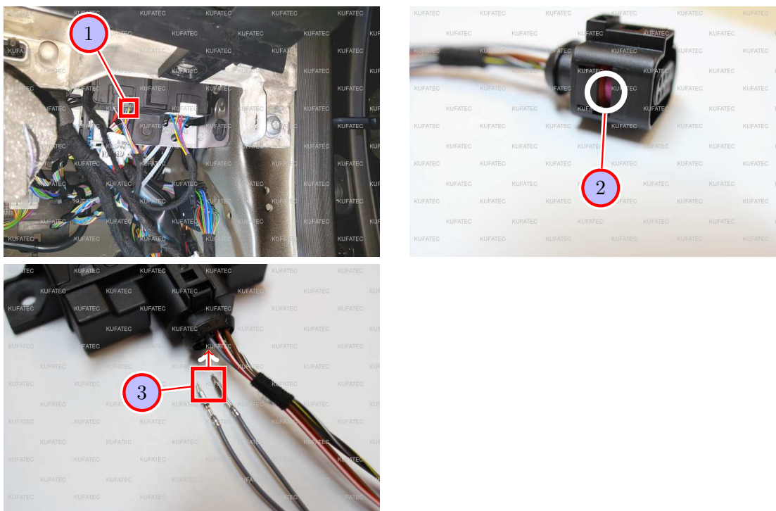
Figure 8: Connection cable set
