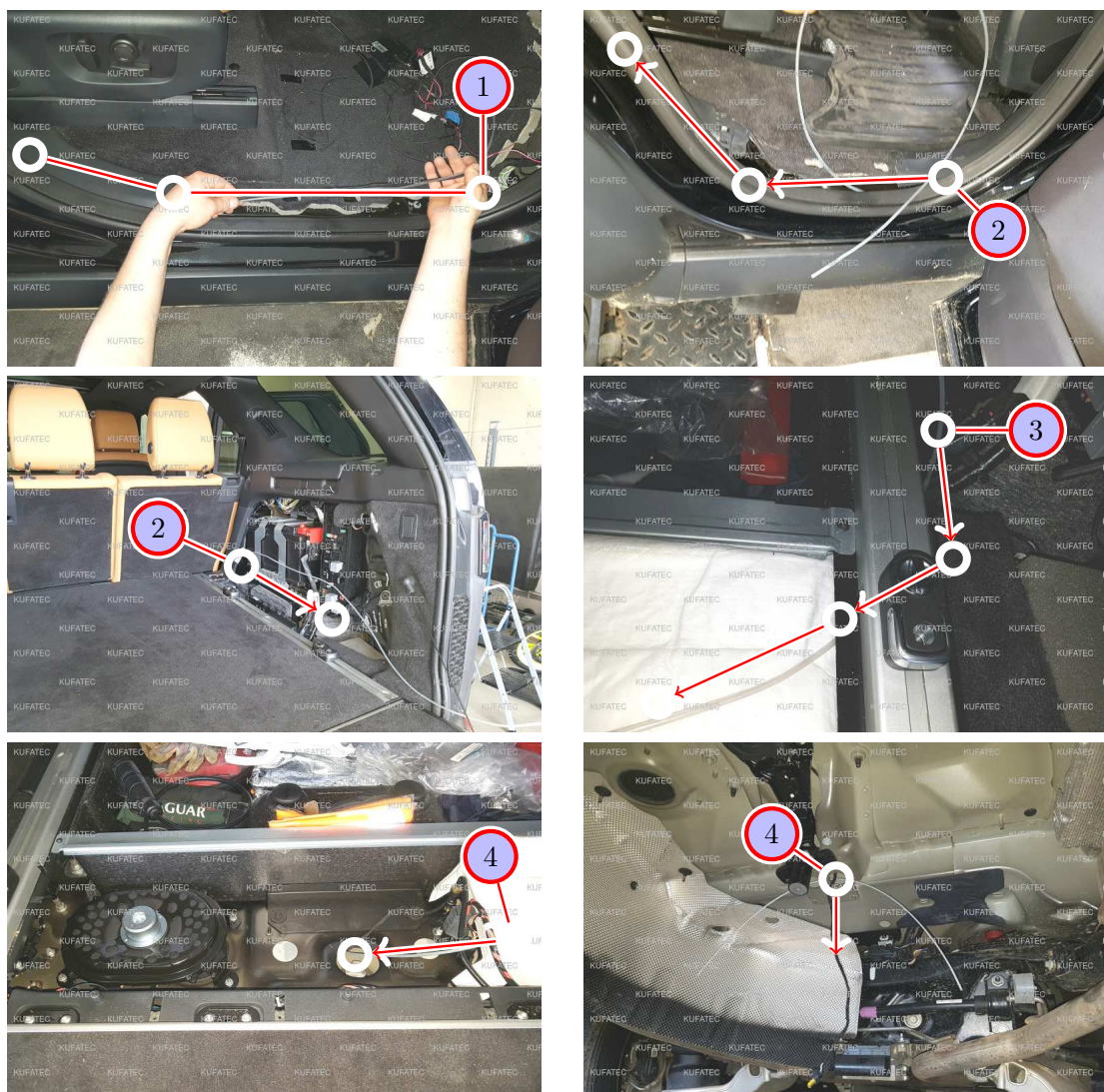
Figure 9: Cable routing to the rear sound generator
