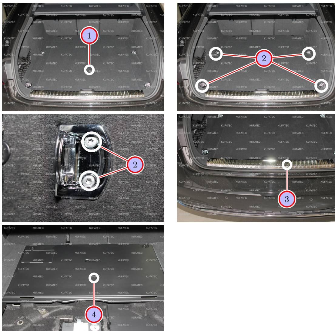
Figure 4: Disassembly trunk
