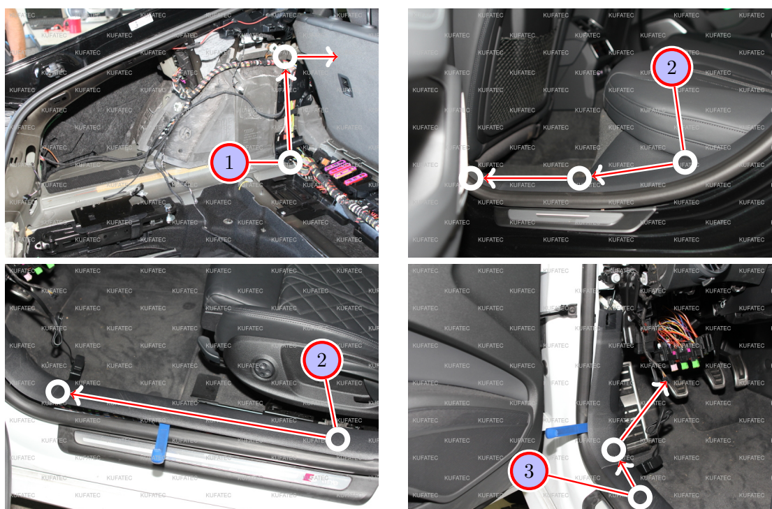
Figure 6: Routing button cable
